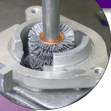
Deburring the internal bores of an air-cooled cylinder head.
